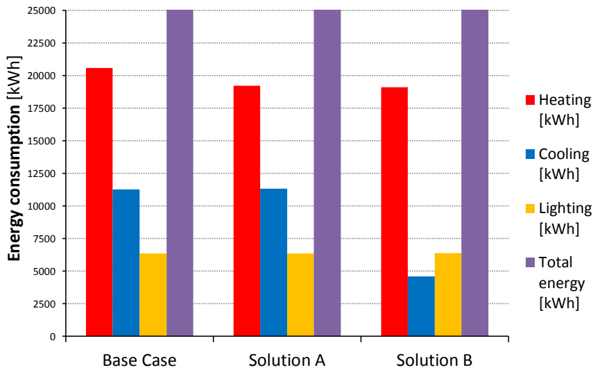
Annual energy consumption by end-use
