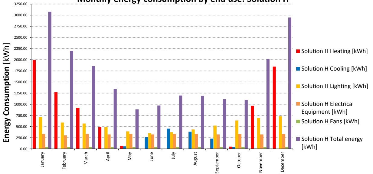
Monthly energy consumption by end-use: Solution H
